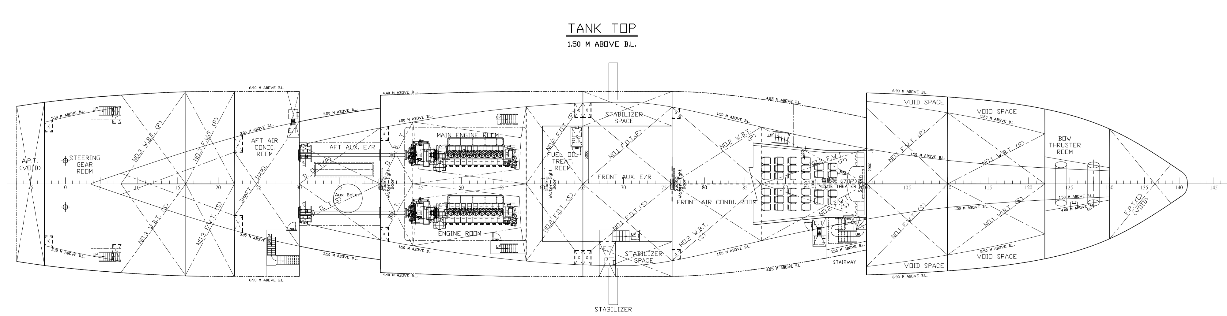
TANK TOP 1.50 M ABOVE BL.
