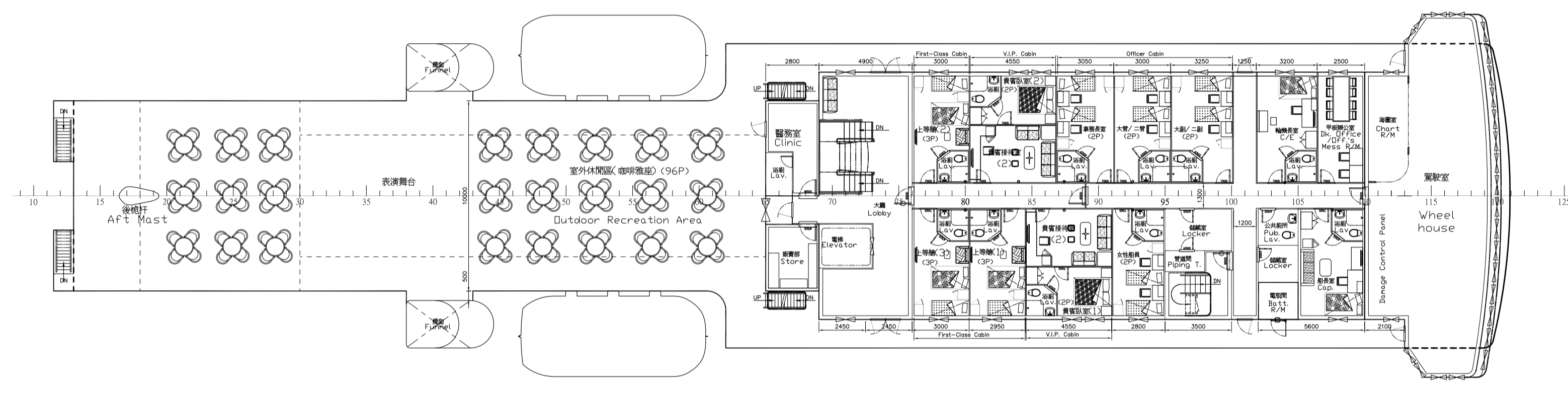
UPPER DECK 12.25 M ABOVE BL. (AT CL)
