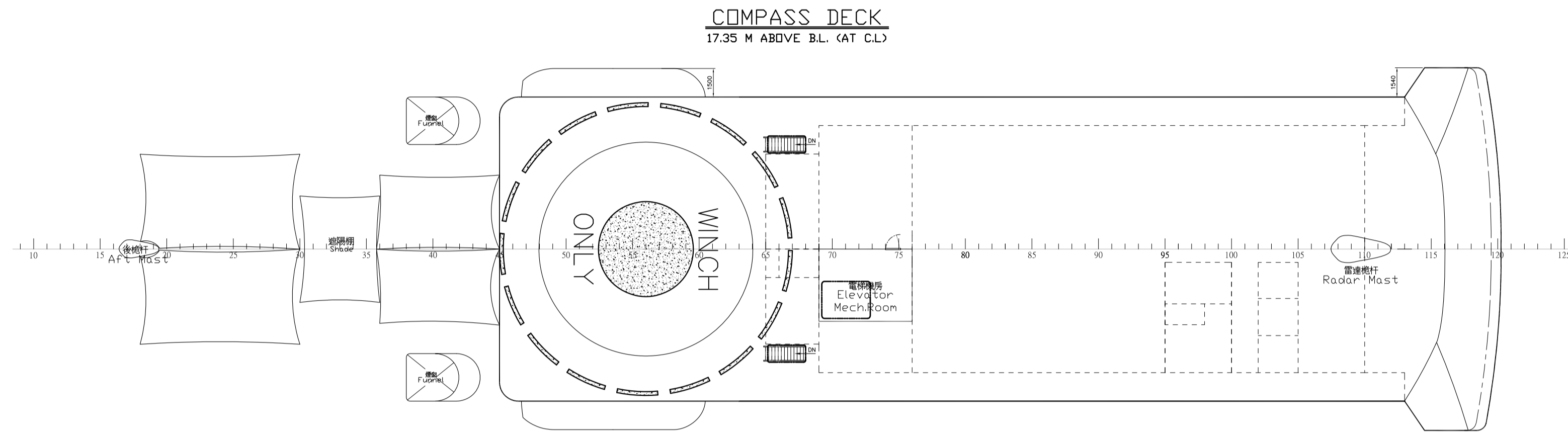
COMPASS DECK 17.25 M ABOVE BL. (AT CL)
